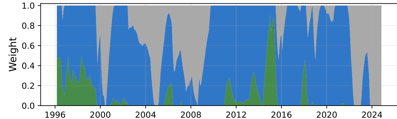
Turnover penalty 0 Sharpe 0.59; turn 91%
